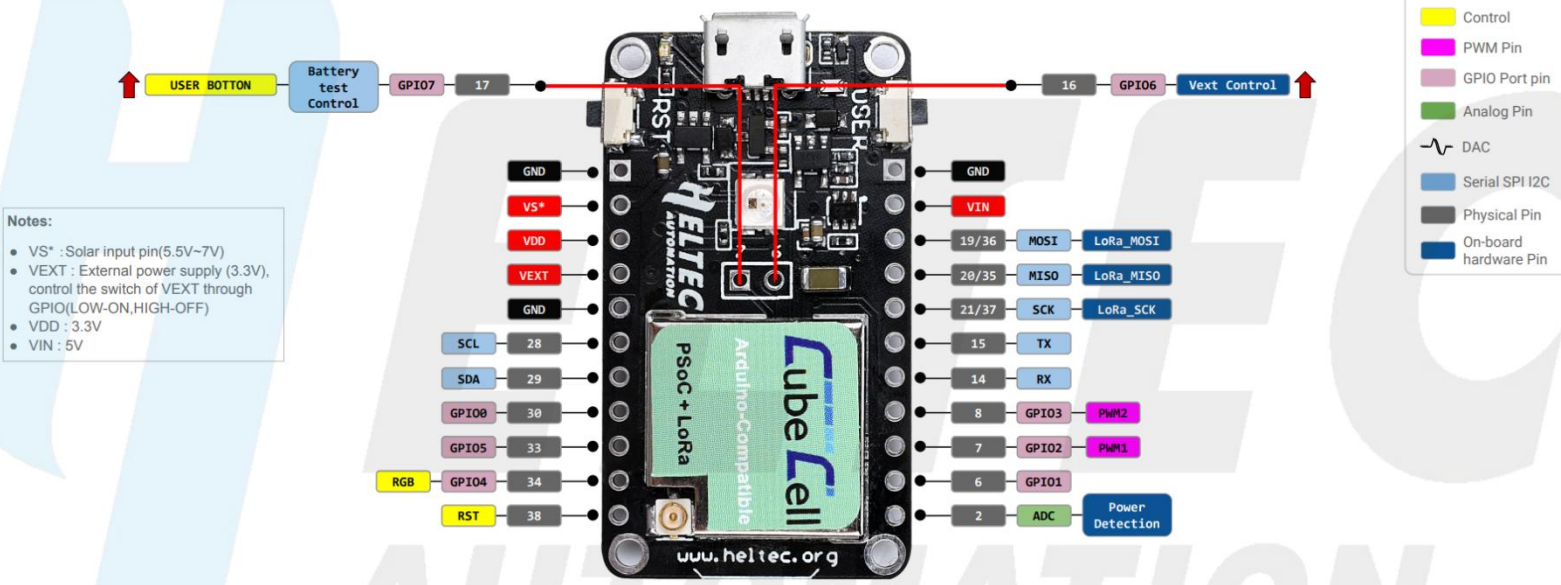
CubeCell HTCC-AB01 Pinout Diagram
