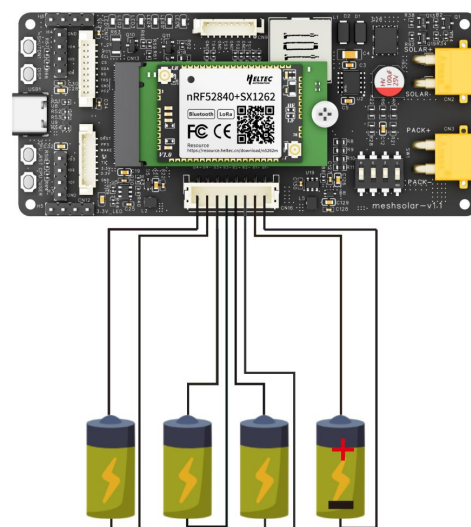
Battery wiring
